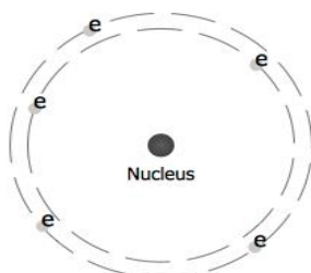
Rutherford-Bohr atom model
