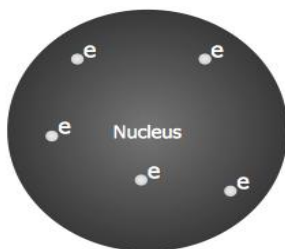
Thompson atom model
